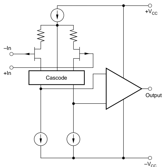
OPA404 Simplified Circuit (Each Amplifier)
