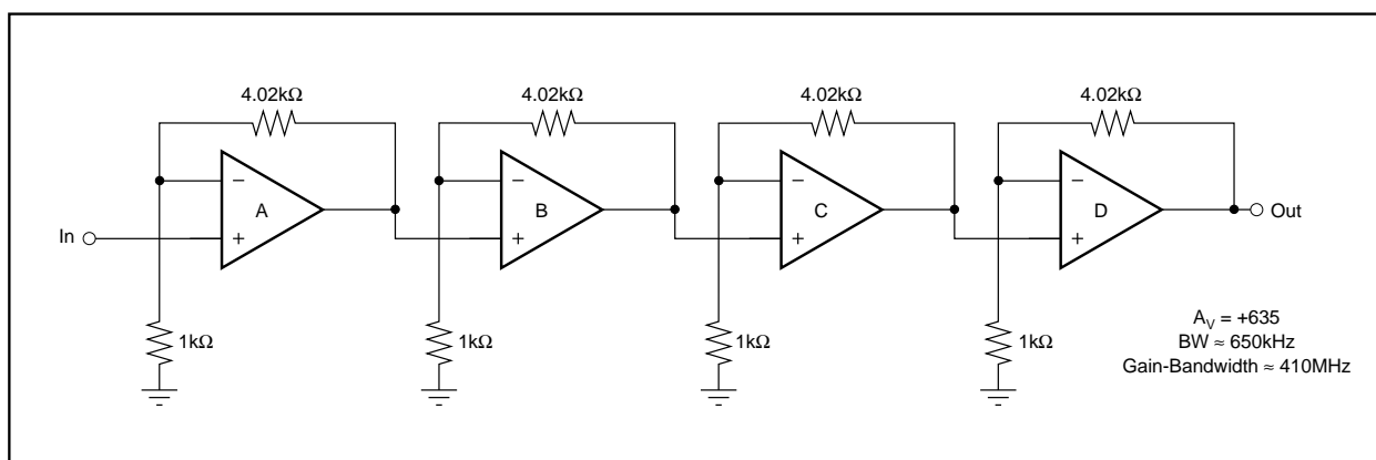
FIGURE 11. Wide-Band Amplifier.
