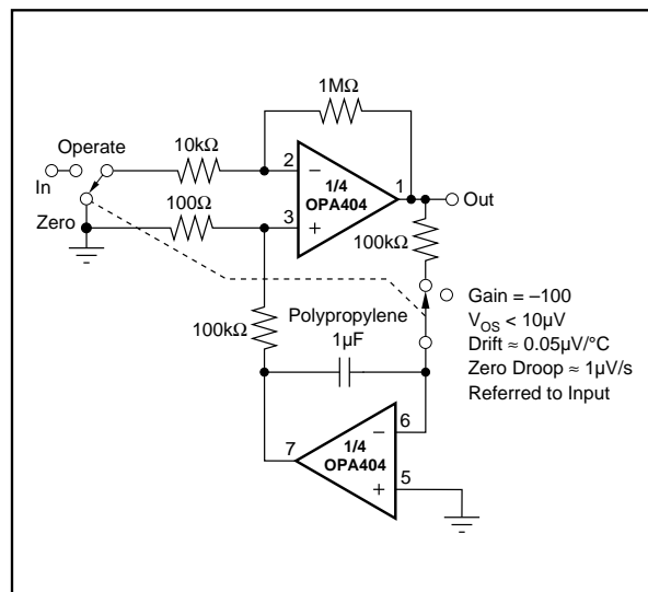
FIGURE 5. Auto-Zero Amplifier.
