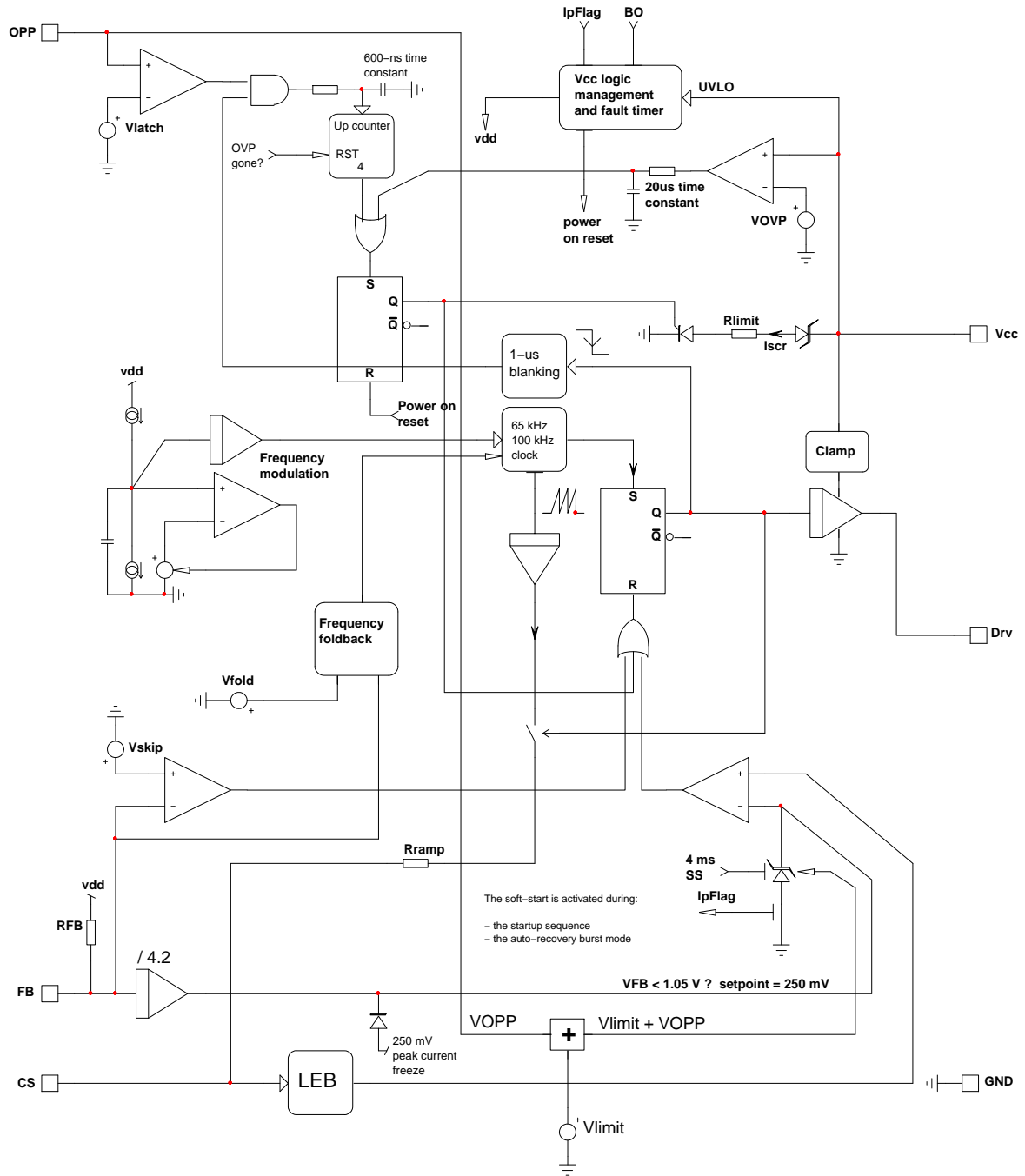
Figure 2. Internal Circuit Architecture
