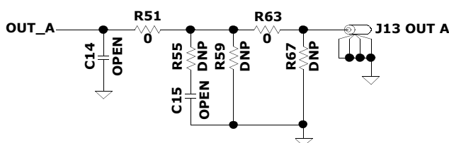
FIGURE 4. OUTPUT STAGE
