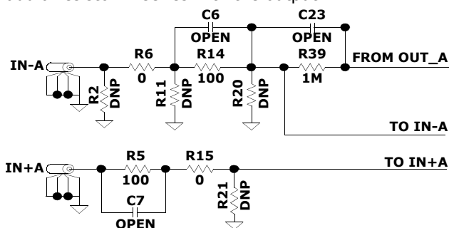
FIGURE 3. INPUT STAGE
