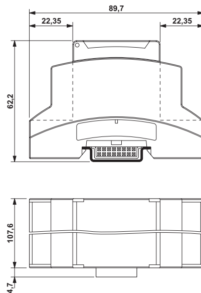
Dimensioned drawing
