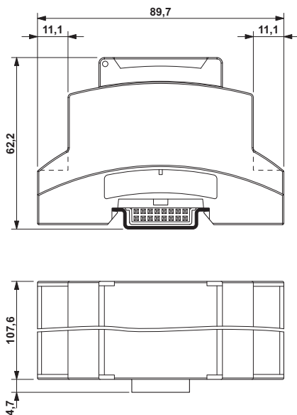
Dimensioned drawing
