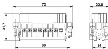
Female insert
