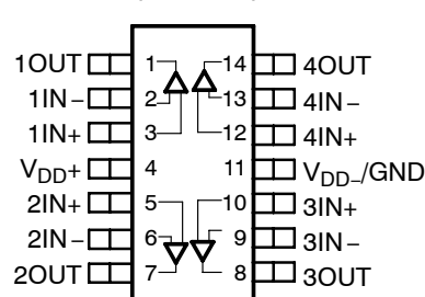
TLV2434 D OR PW PACKAGE (TOP VIEW)
