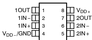
TLV2432 D PACKAGE (TOP VIEW)
