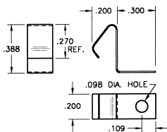
CAT. NO. 5230 CAT. NO. 5230TR
