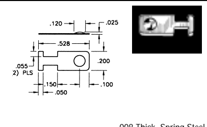
CAT. NO. 230-1 .008 Thick, Spring Steel, Nickel Plate
