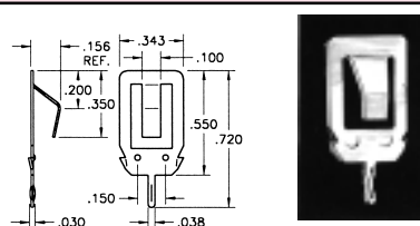
CAT. NO. 108-2 .012 Thick, Spring Steel, Nickel Plate
