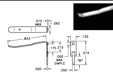
CAT. NO. 105-2 .020 Thick, Spring Steel, Nickel Plate
