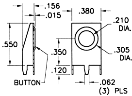
Mounting Detail
