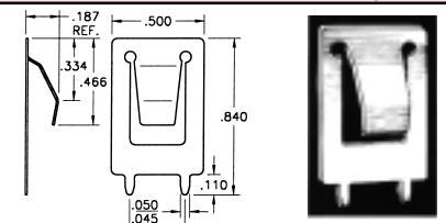
CAT. NO. 109-2 .012 Thick, Spring Steel, Nickel Plate
