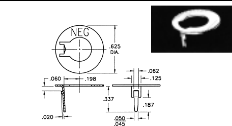
CAT. NO. 105-3 .020 Thick, Spring Steel, Nickel Plate
