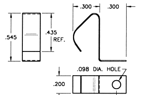
Tape and Reel Spec's: 32mm wide; 12mm pitch; 13 inch reel (400 pieces per reel)
