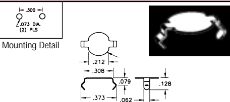
CAT. NO. 2990 .008 Thick, Phosper Bronze, Nickel Plate
