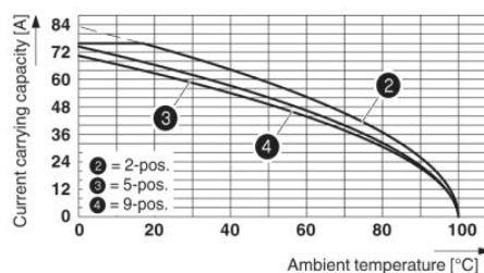
Derating curve for: IPC 16/...-ST-10,16 with IPC 16/...-G-10,16
