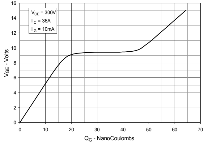
Fig. 8. Gate Charge
