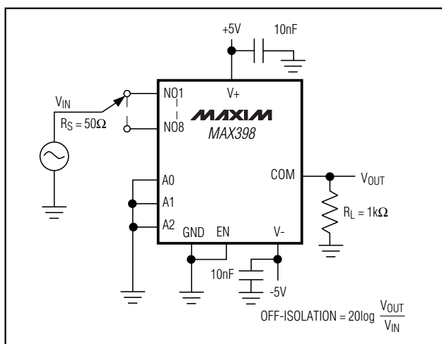
Figure 6. Off-Isolation
