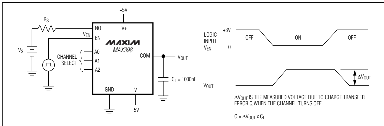
Figure 5. Charge Injection
