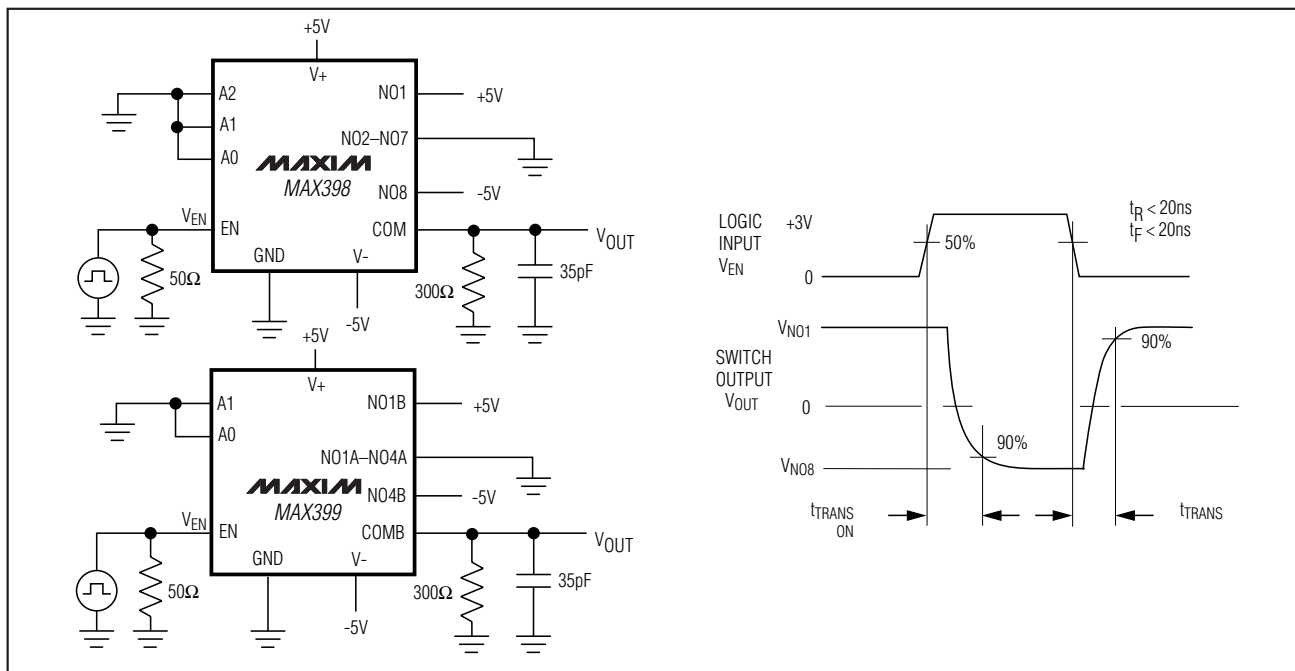
Figure 2. Transition Time
