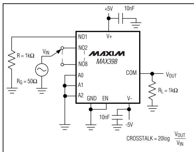
Figure 7. Crosstalk
