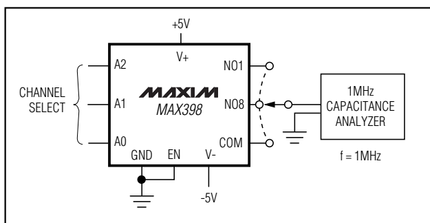
Figure 8. NO/COM Capacitance
