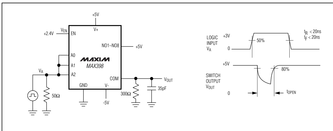
Figure 4. Break-Before-Make Interval
