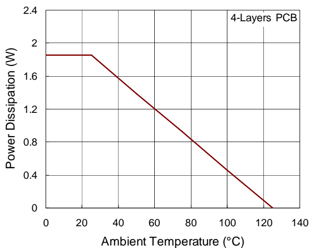
Figure 3. De-rating Curve
