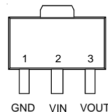
RT9162-33xXL RT9162-35xXL SOT-89
