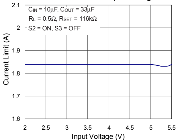
③ Current Limit vs. Input Voltage
