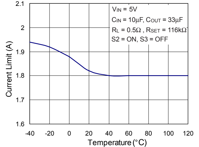
③ Current Limit vs. Temperature
