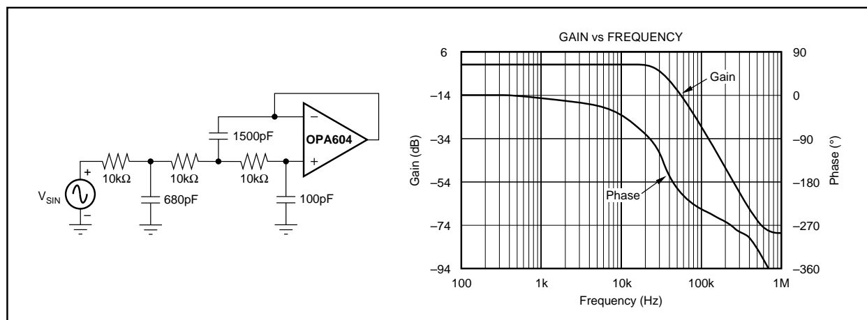
FIGURE 13. 3rd-Order LPF.
