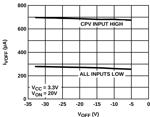
FIGURE 3. V_{OFF} DC SUPPLY CURRENT vs V_{OFF}
