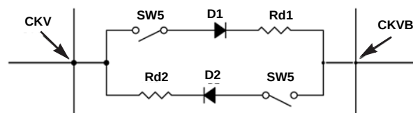
FIGURE 18. BI-DIRECTIONAL SWITCHES
