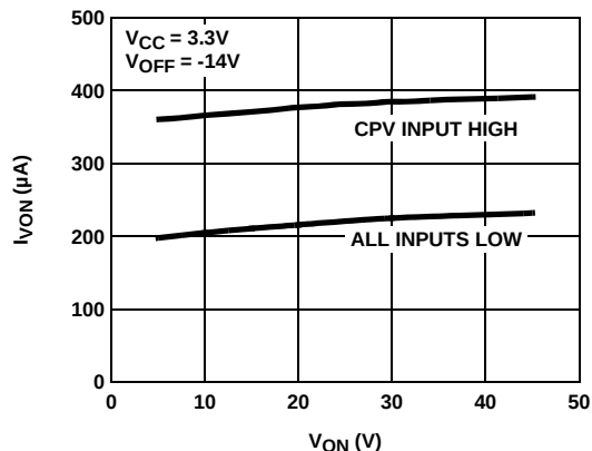
FIGURE 2. V_{ON} DC SUPPLY CURRENT vs V_{ON}
