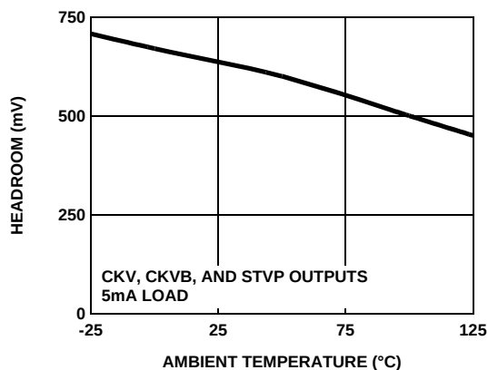
FIGURE 10. OUTPUT SWING HEADROOM vs TEMPERATURE
