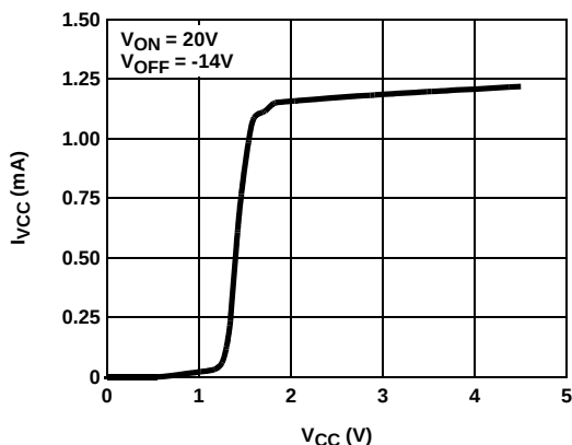
FIGURE 1. V_{SS} SUPPLY CURRENT vs V_{CC}
