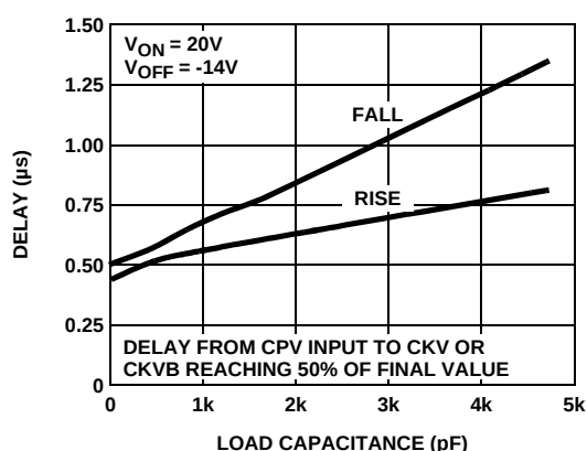
FIGURE 4. CLOCK DELAY vs LOAD CAPACITOR
