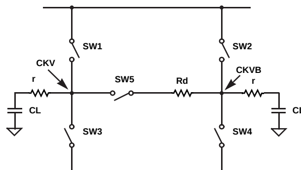
FIGURE 17. BI-DIRECTIONAL SWITCHES
