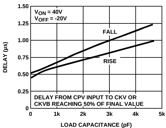
FIGURE 5. CLOCK DELAY vs LOAD CAPACITOR
