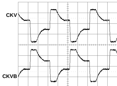
FIGURE 21. CKV AND CKVB OUTPUT WAVEFORMS
