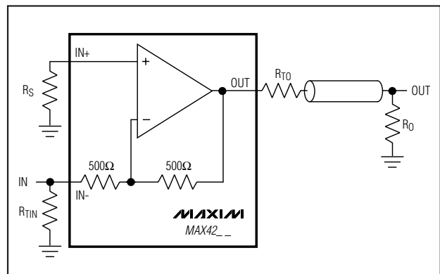
Figure 1b. Inverting Gain Configuration ( A_V = -1V/V )
