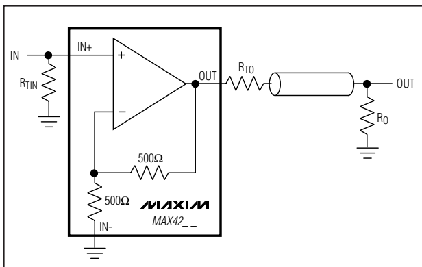
Figure 1a. Noninverting Gain Configuration ( A_V = +2V/V )
