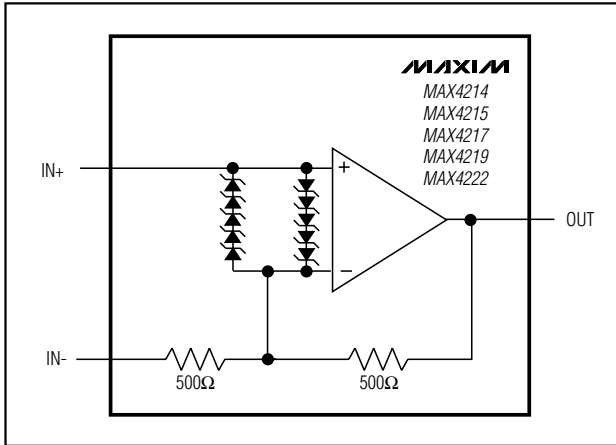
Figure 5. Input Protection Circuit
