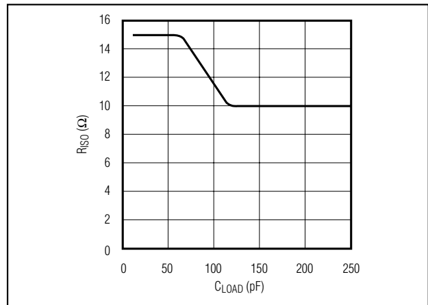
Figure 8. Isolation Resistance vs. Capacitive Load
