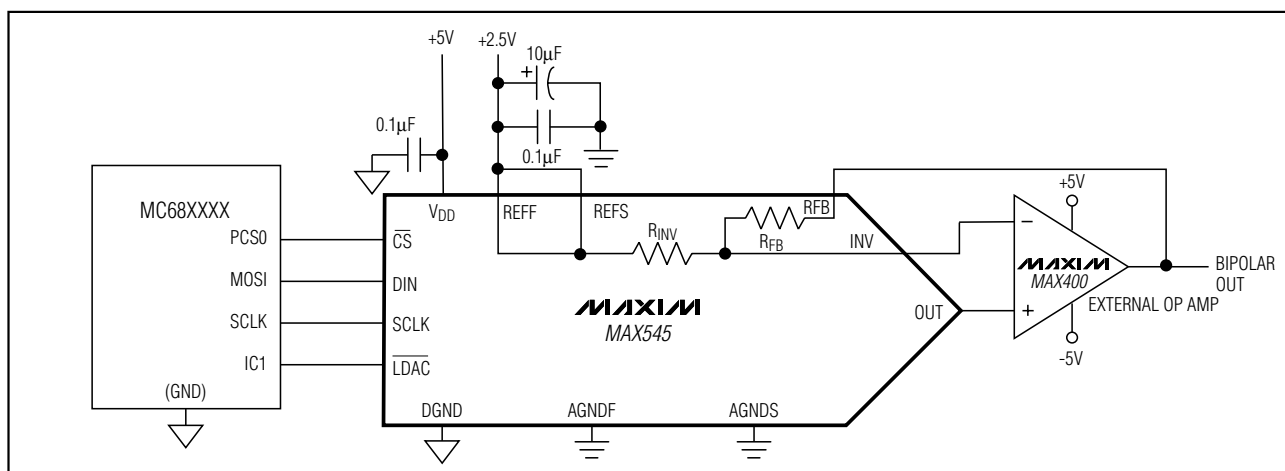
Figure 2b. Typical Operating Circuit—Bipolar Output
