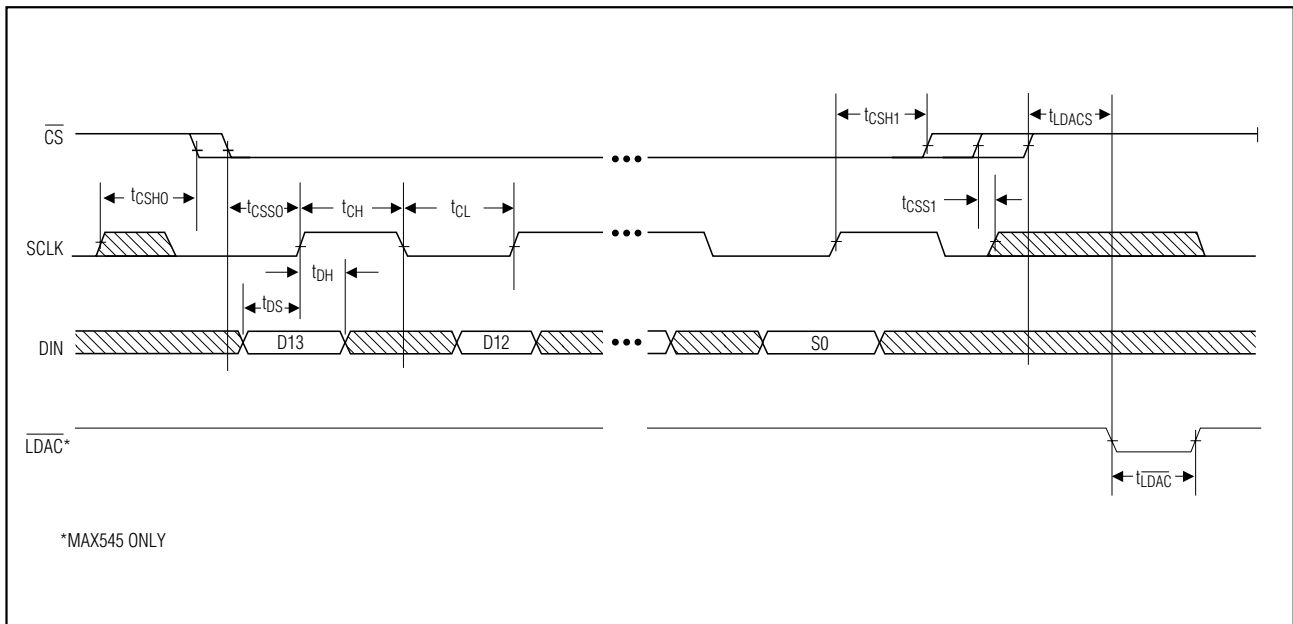
Figure 1. Timing Diagram
