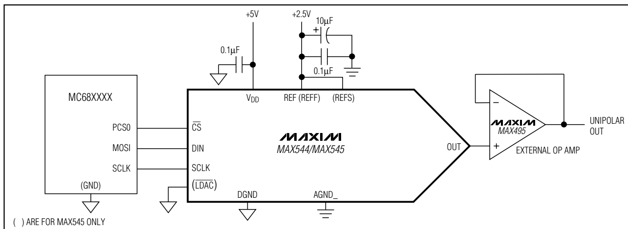
Figure 2a. Typical Operating Circuit—Unipolar Output
