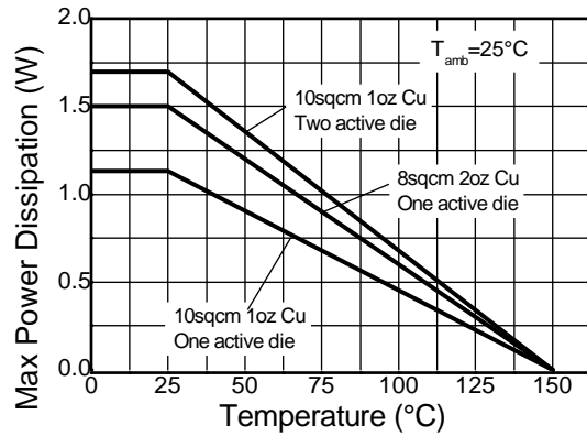
Derating Curve
