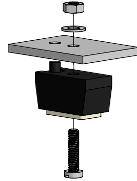
EXPLODED ASSEMBLY VIEW (PLATE NOT INCLUDED)
