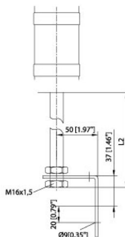
Threaded Tubular Stand/Bracket
