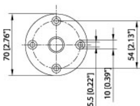
Tubular Stand/Plinth
