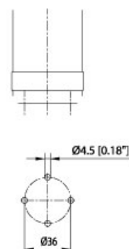
Direct Mounting
