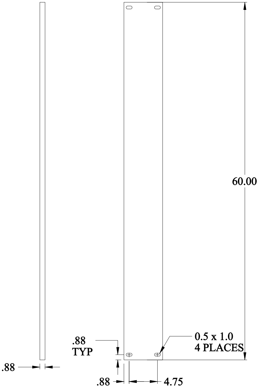
FORMED VIEW
