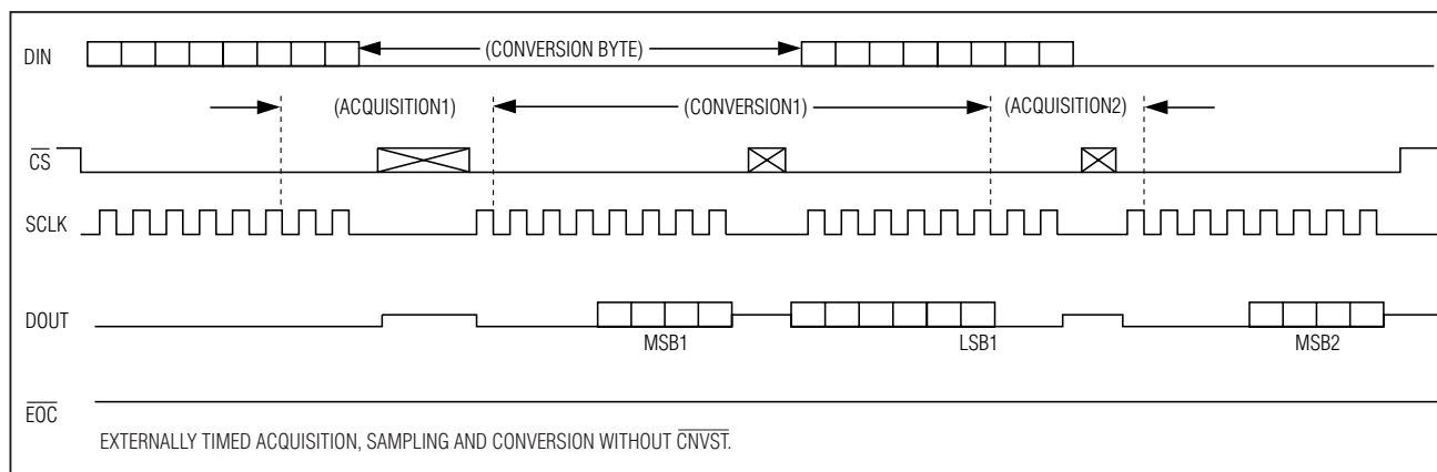
Figure 7. Clock Mode 11
