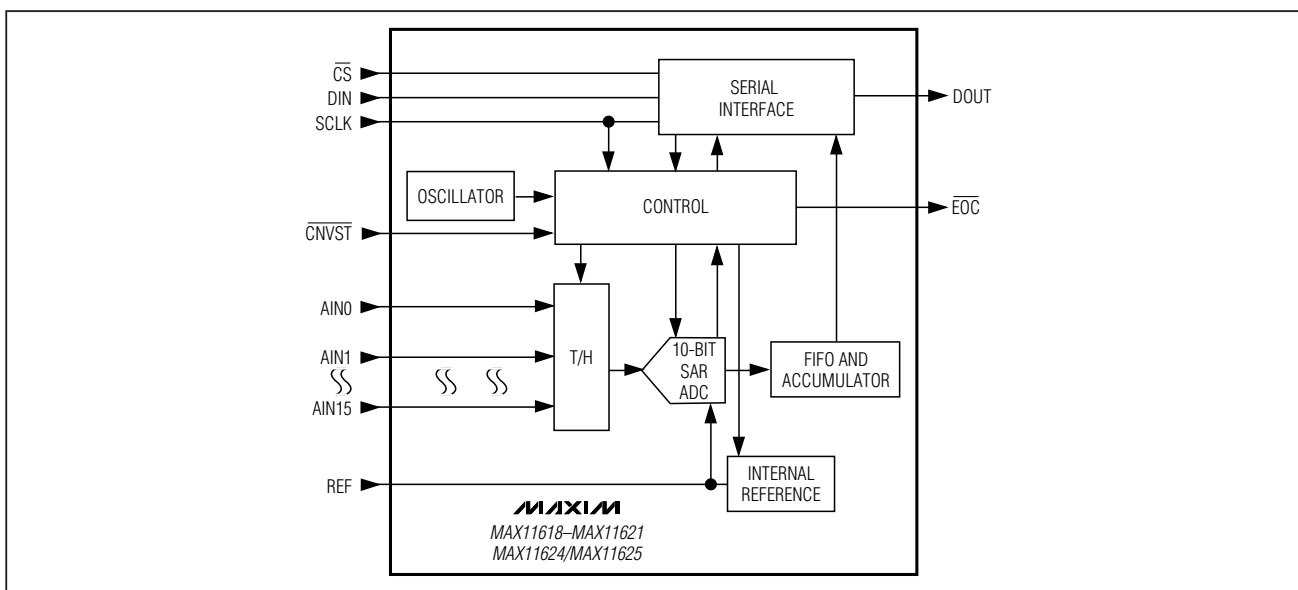
Figure 2. Functional Diagram
