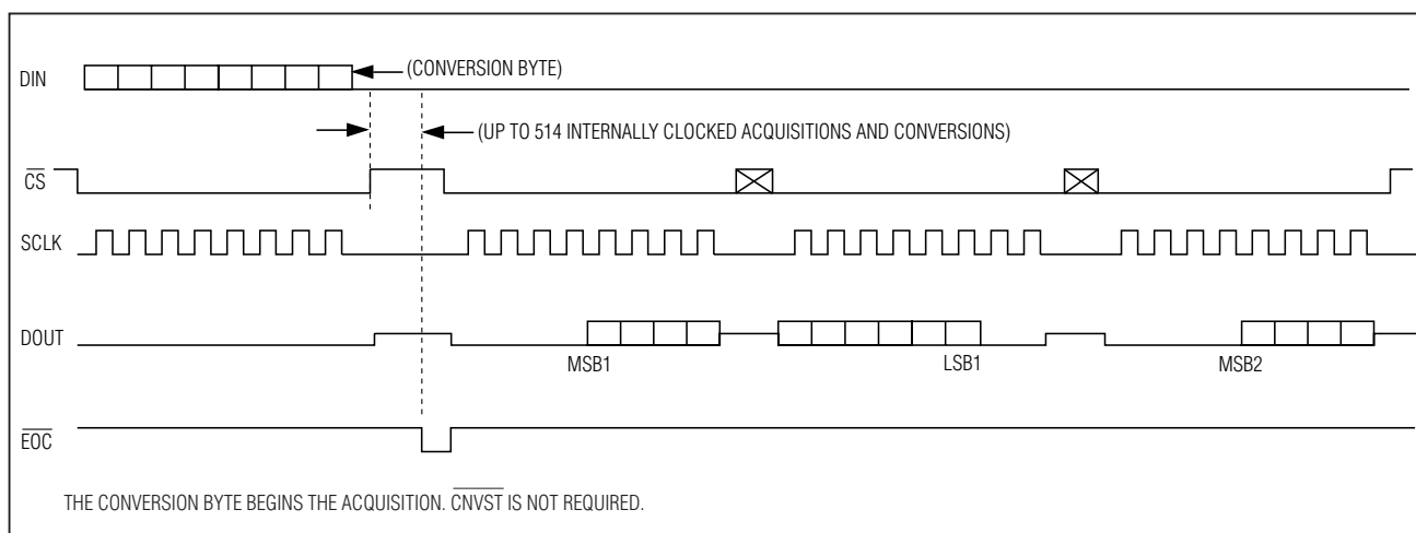
Figure 6. Clock Mode 10
