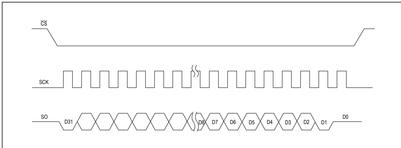
Figure 1. Serial-Interface Protocol
