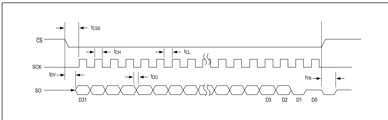
Figure 2. Serial-Interface Timing
