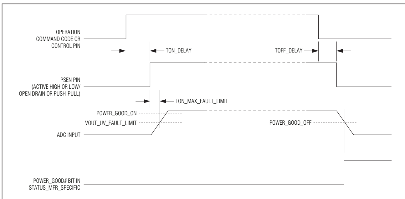
Figure 4. Power-Supply Sequencing
