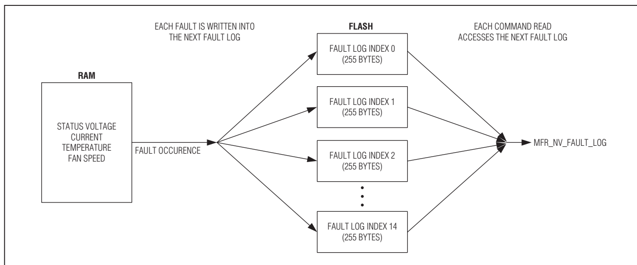
Figure 5. MFR_NV_FAULT_LOG
