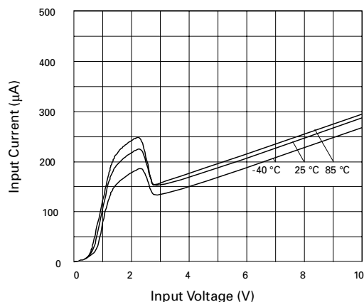
Input Current vs. Input Voltage
