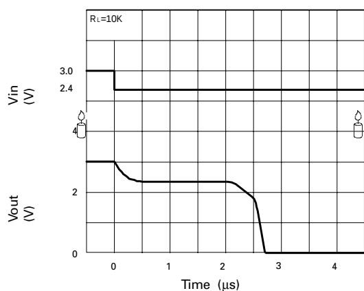
Reset Delay Time
