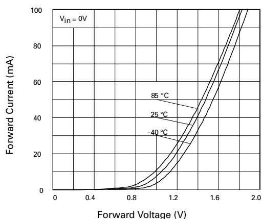
Clamp Diode Forward Current vs. Voltage
