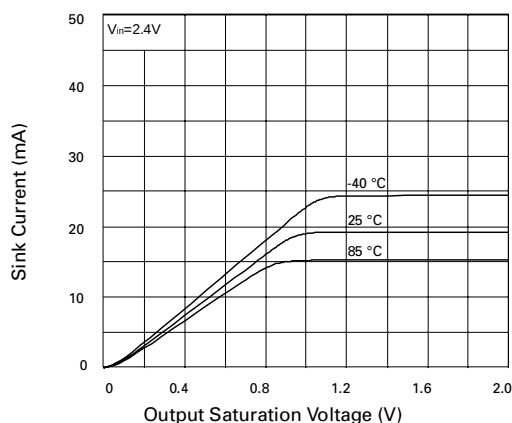
Output Saturation Voltage vs. Sink Current
