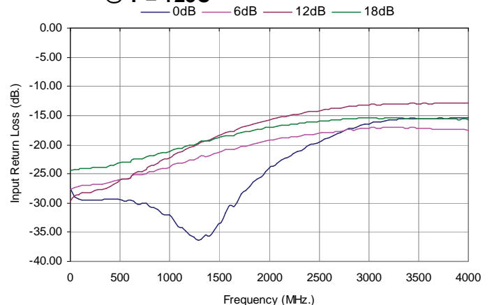
Figure 6. Input Return Loss vs Attenuation @ T = +25C
