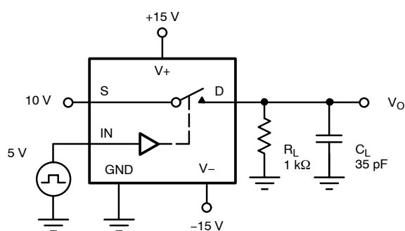
FIGURE 2. Switching Time
