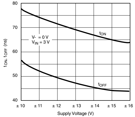
Switching Time vs. Supply Voltages
