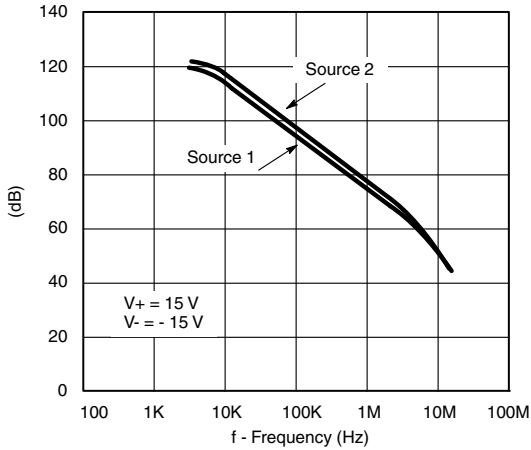
Crosstalk and Off Isolation vs. Frequency
