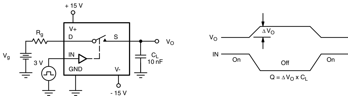
Fig. 7 - Charge Injection
