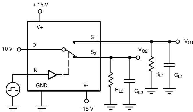
Fig. 3 - Break-Before-Make
