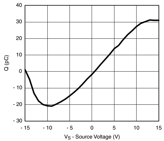
Drain Charge Injection
