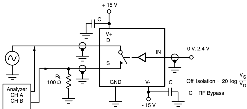
Fig. 4 - Off Isolation
