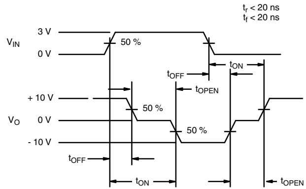
Fig. 2 - Switching Time
