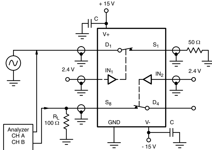
Fig. 5 - Crosstalk
