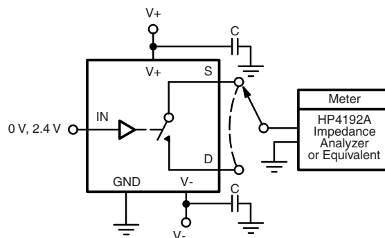
Figure 6. Source/Drain Capacitances
