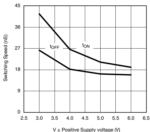
Switching Time vs. Dual Supply
