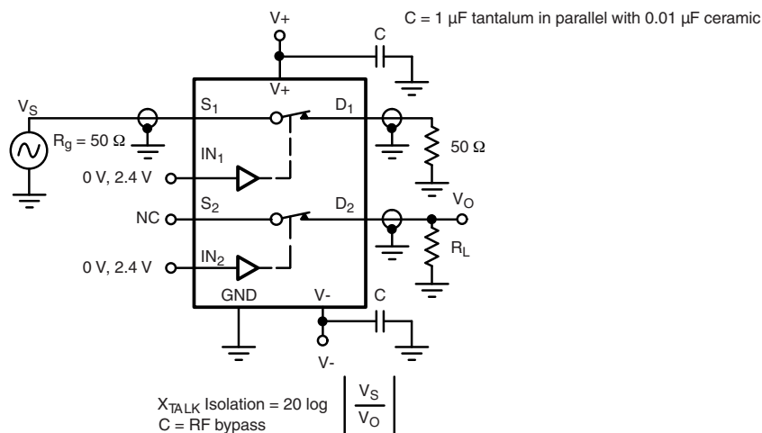
Figure 4. Crosstalk
