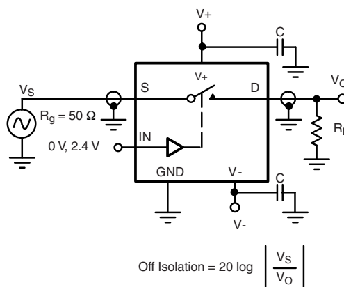
Figure 5. Off Isolation
