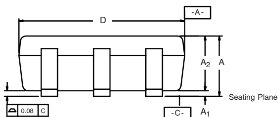
5-LEAD TSOP
