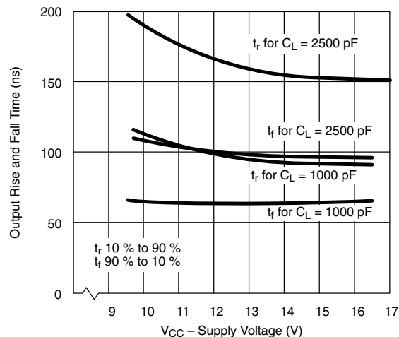
Output Driver Rise and Fall Time
