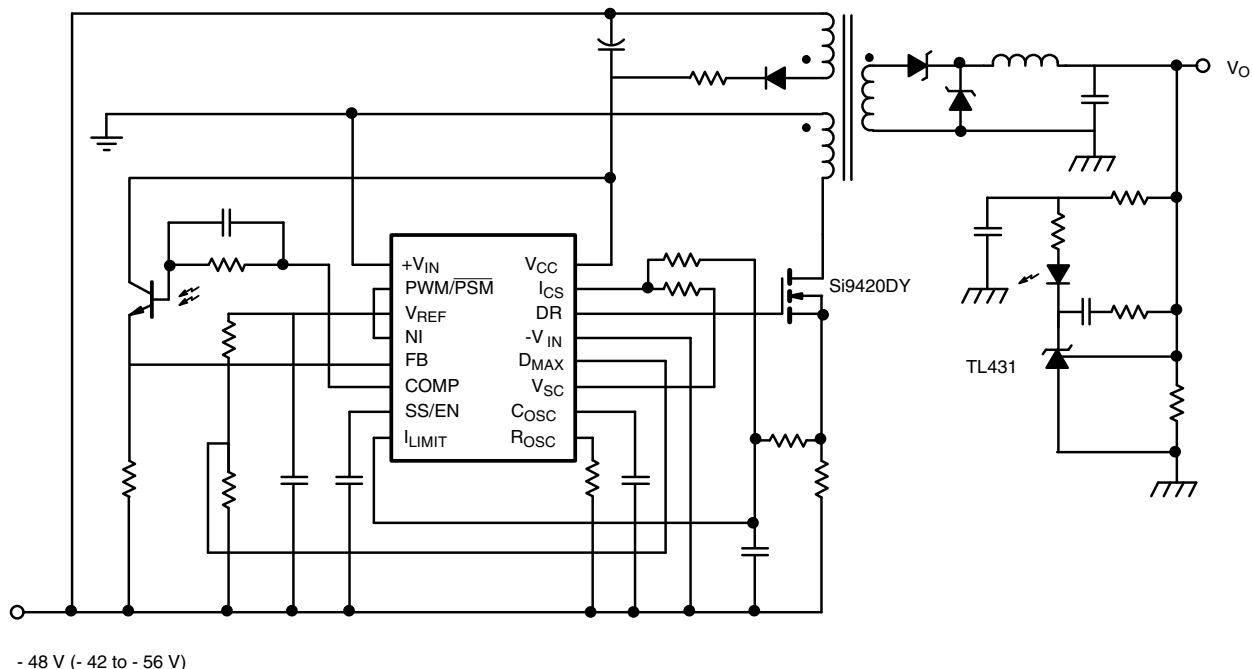
Figure 2. Si9118 15 W Forward Converter Schematic
