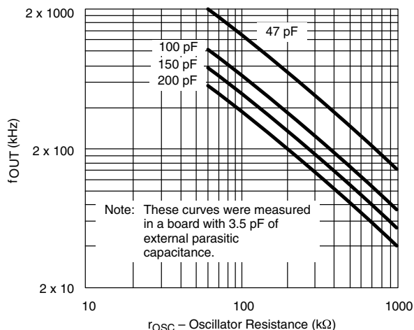
Oscillator Frequency
