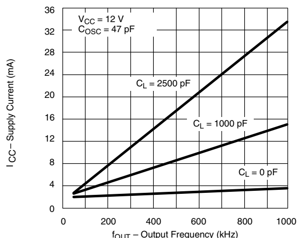
Supply Current vs. Output Frequency
