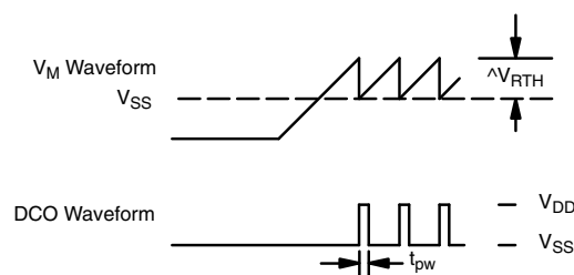
Figure 7. Load Detection in Overcharge Mode
