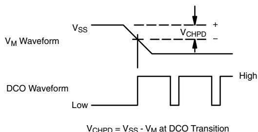
Figure 6. Power-Down Charger Detect Threshold
