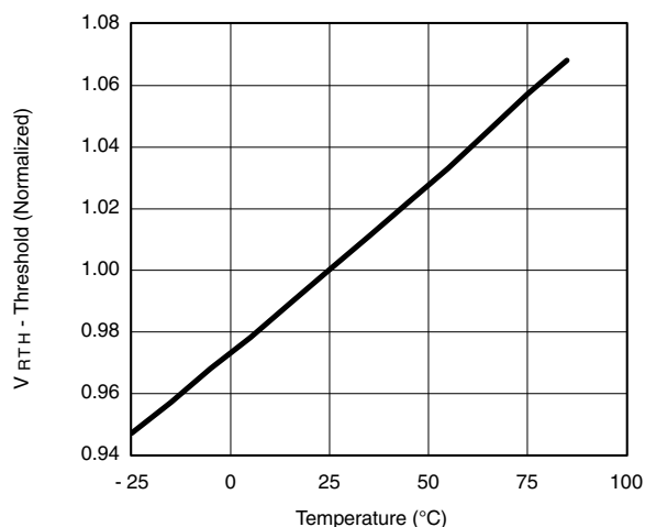
Reset Threshold vs. Temperature
