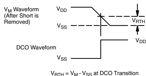
Figure 3. Reset Threshold
