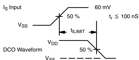
Figure 2. Current-Limit Comparator Response Time
