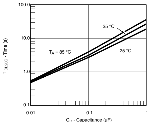
DL2 Period (Over Discharge) vs. Capacitance
