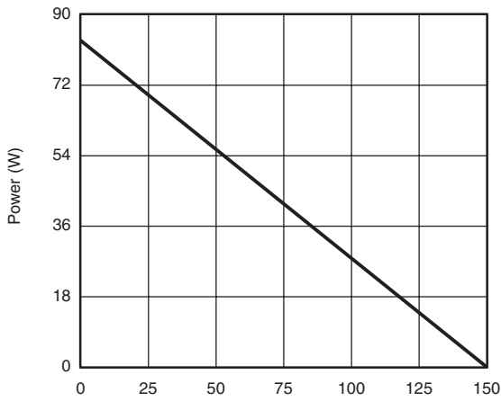
Power, Junction-to-Case
