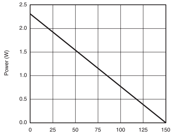
Power, Junction-to-Ambient
