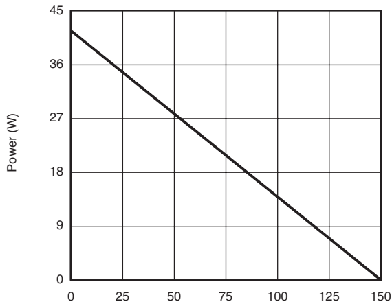
Power, Junction-to-Case
