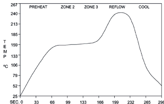
Fig. 3 Solder Reflow Temperature Profile
