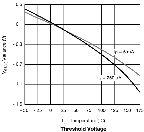
Threshold Voltage
