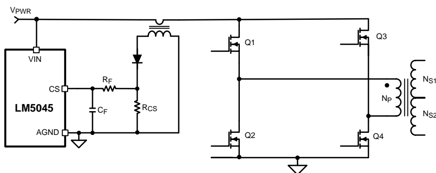
Figure 27. Transformer Current Sense
