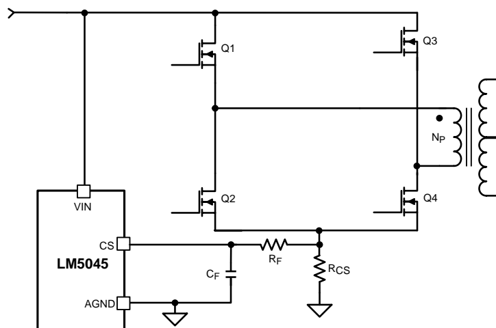
Figure 28. Resistor Current Sense
