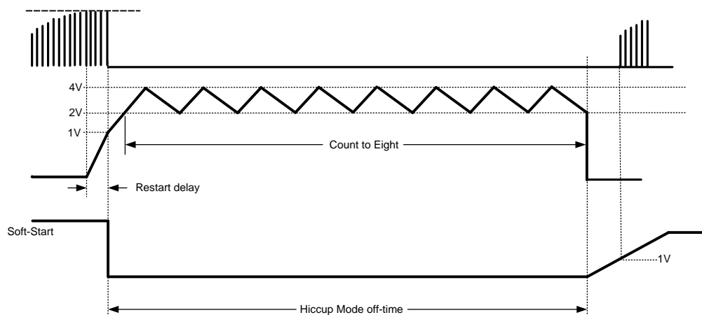
Figure 10. Hiccup Mode Delay and Soft-Start Timing Diagram
