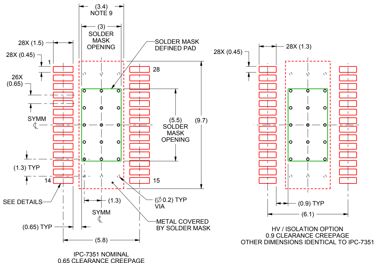
LAND PATTERN EXAMPLE SCALE:6X
