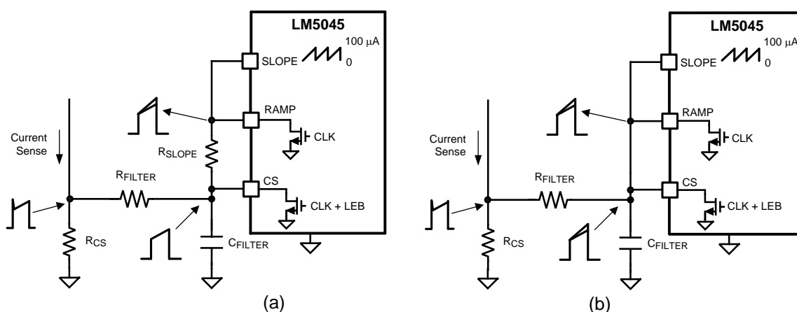
Figure 11. Slope Compensation Configuration
