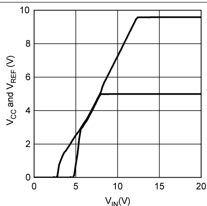
Figure 3. V_{CC} and V_{REF} vs V_{IN}
