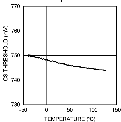
Figure 9. CS Threshold vs Temperature
