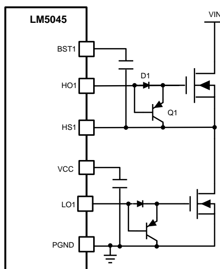
Figure 30. Circuit to Speed-Up the Turnoff Process
