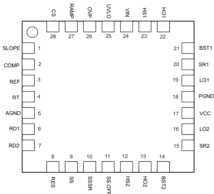
RSG Package 28-Pin WQFN, 5 mm x 5 mm Top View
