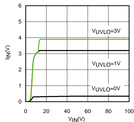
Figure 4. I_{IN} vs V_{IN}
