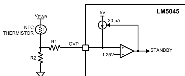
Figure 26. Remote Thermal Protection
