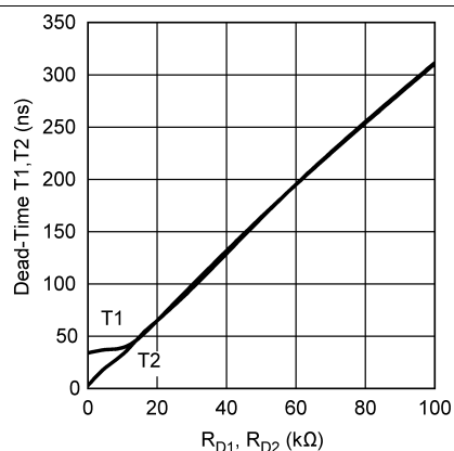
Figure 7. Dead-Time T1, T2 vs R_{D1} , R_{D2}
