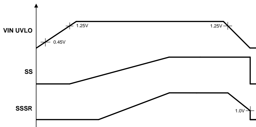
Figure 16. Stop-Stop Waveforms During a UVLO Event
