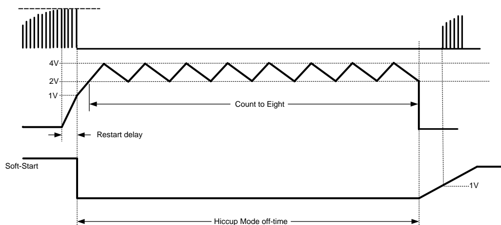
Figure 29. Hiccup Mode Delay and Soft-Start Timing Diagram
