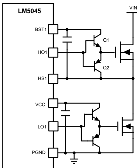
Figure 31. Bipolar Totem Pole Arrangement
