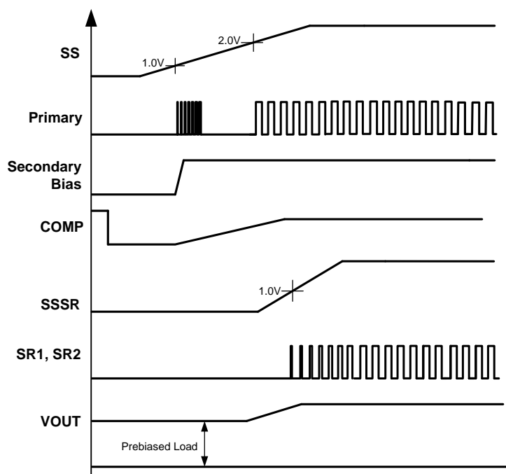
Figure 15. Prebias Voltage Start-up Waveforms
