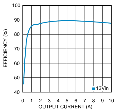
Figure 50. Efficiency
