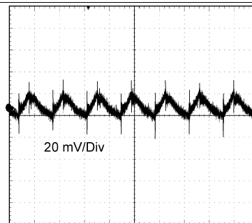
Figure 34. Output Ripple
