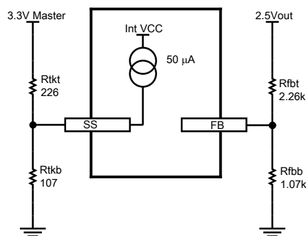
Figure 49. Tracking Option Input Detail
