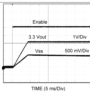
Figure 44. 3.3 V OUT Soft-Start
