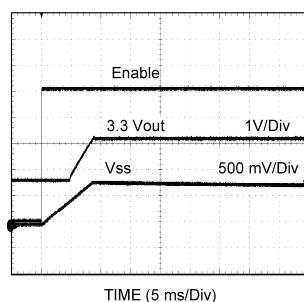
Figure 45. Prebiased Start-Up
