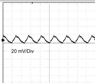
Figure 33. Output Ripple
