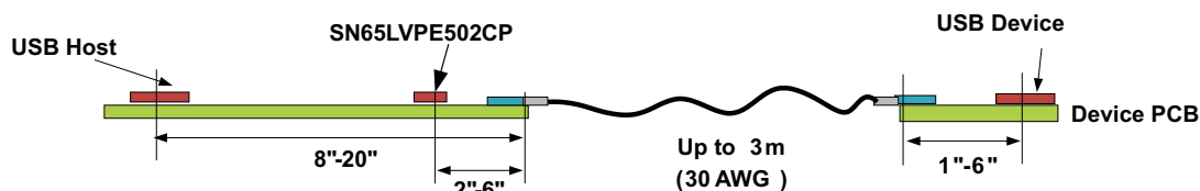
Figure 9. Redriver Placement Example
