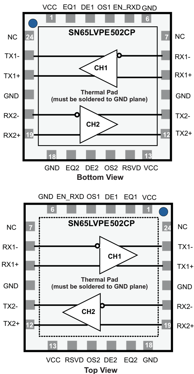
Figure 8. Flow-Through Pin-Out
