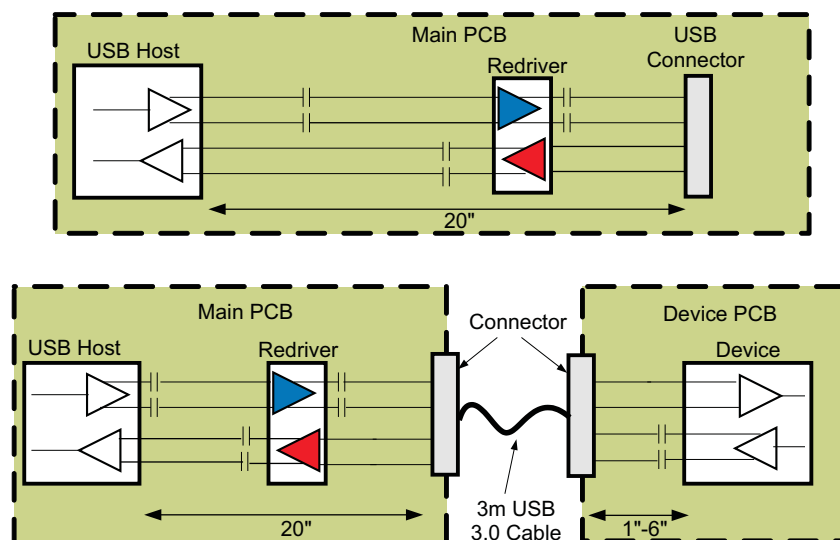
Figure 1. Typical Application
