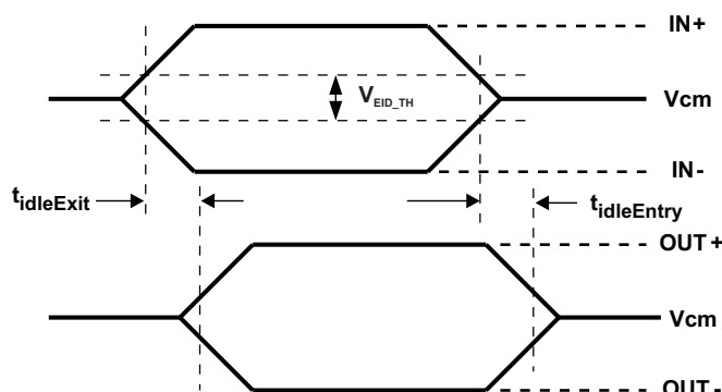
Figure 4. Electrical Idle Mode Exit and Entry Delay
