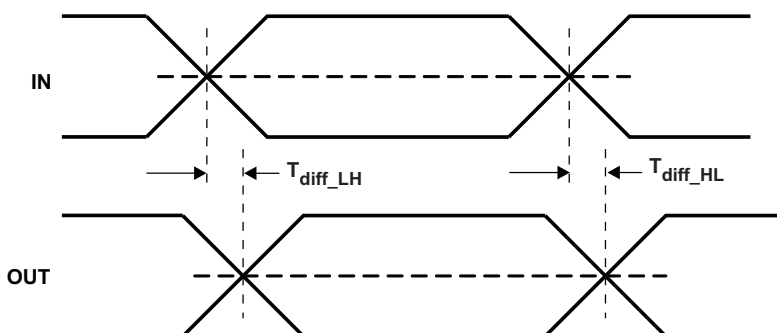
Figure 3. Propagation Delay
