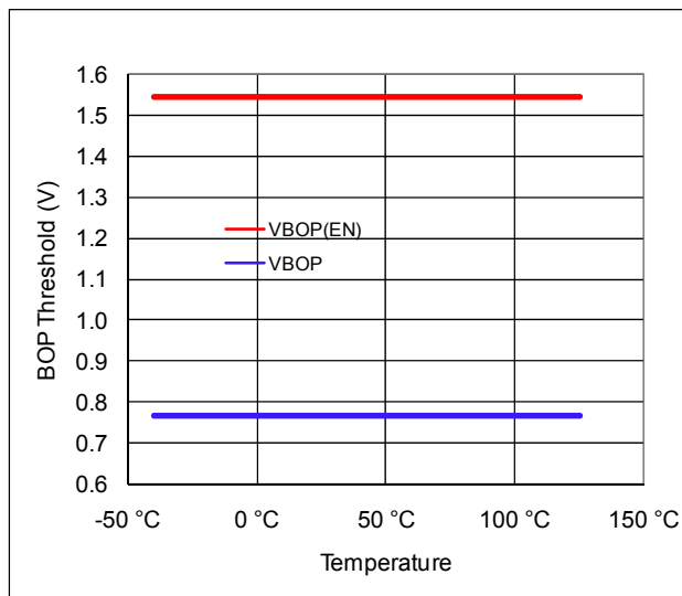
Figure 12: Brown-Out Protection Thresholds vs. Temperature
