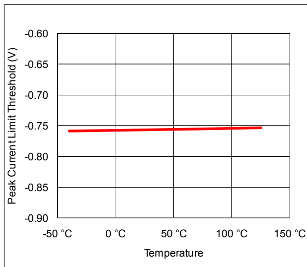
Figure 10: Peak Current Limit Threshold V_{ISNS(PK)} vs. Temperature
