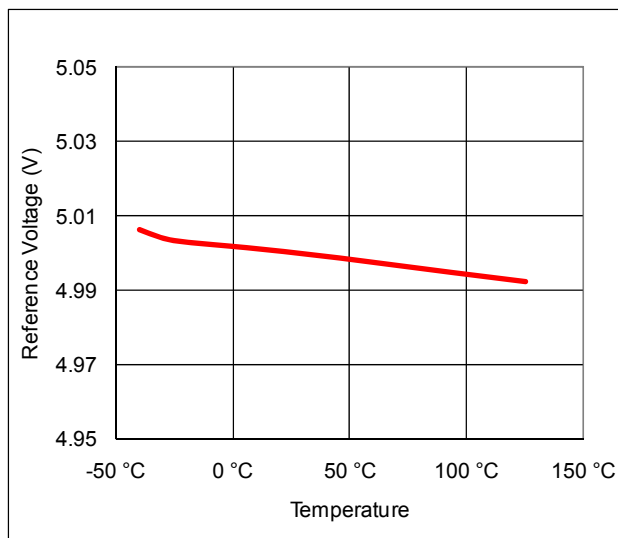
Figure 6: Reference Voltage vs. Temperature
