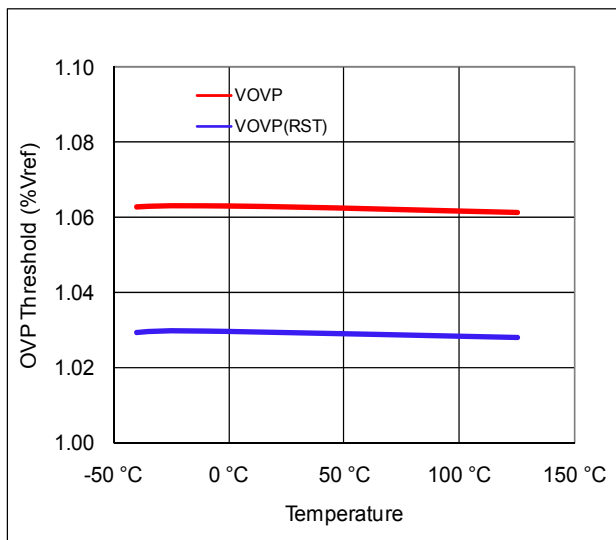
Figure 11: Over Voltage Protection Thresholds vs. Temperature
