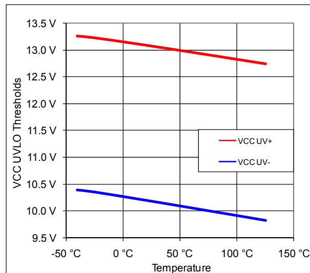
Figure 2: Undervoltage Lockout vs. Temperature
