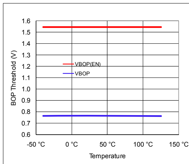
Figure 12: Brown-Out Protection Thresholds vs. Temperature
