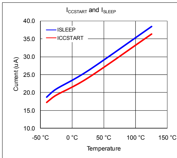
Figure 4: Startup Current and Sleep Current vs. Temperature
