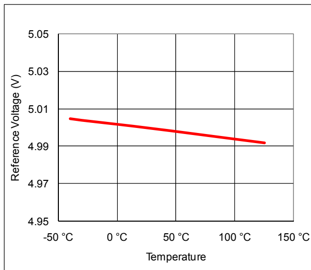
Figure 6: Reference Voltage vs. Temperature
