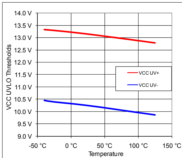
Figure 2: Undervoltage Lockout vs. Temperature
