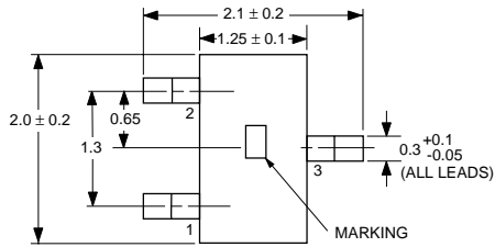
PACKAGE OUTLINE 30
