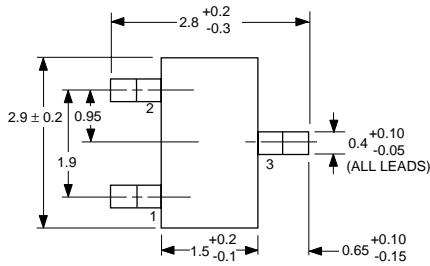
PACKAGE OUTLINE 33
