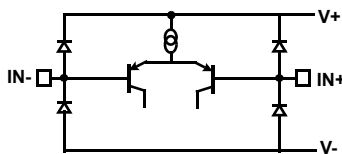
CIRCUIT 1
