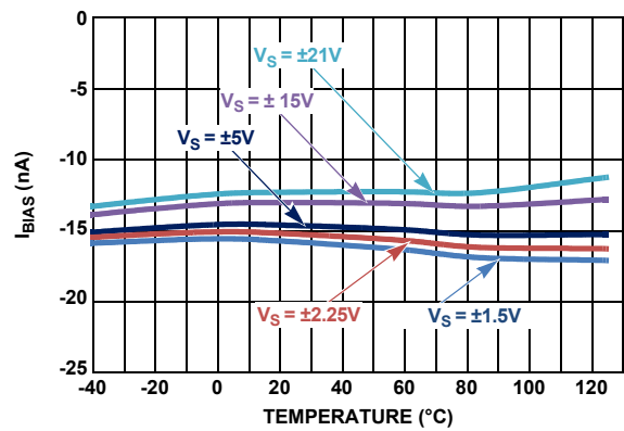
FIGURE 22. I_{BIAS} vs TEMPERATURE vs SUPPLY
