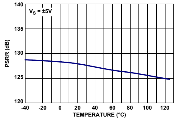
FIGURE 30. PSRR (DC) vs TEMPERATURE, V_S = \pm 5V
