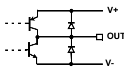
CIRCUIT 2
