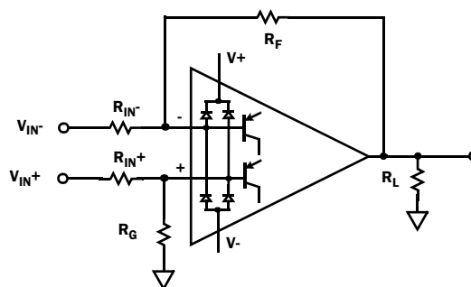
FIGURE 65. INPUT ESD DIODE CURRENT LIMITING
