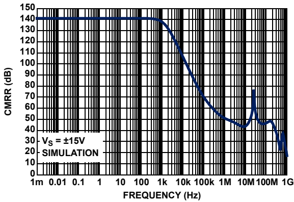
FIGURE 27. CMRR vs FREQUENCY, V_S = \pm 15V
