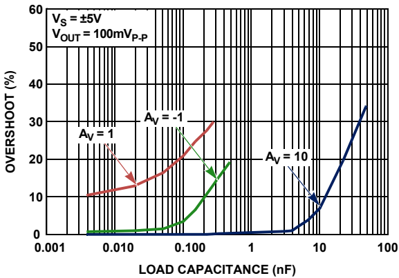
FIGURE 61. OVERSHOOT vs CAPACITIVE LOAD, V_S = \pm 5V
