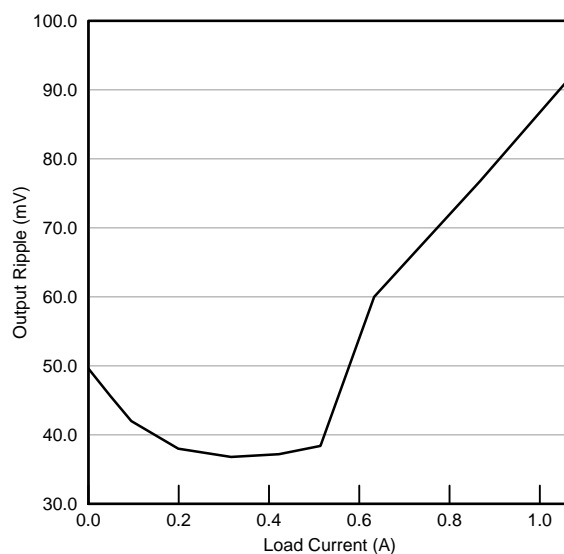
Figure 9. Output Ripple vs. I_{LOAD} ( C_{OUT} = 1\mu F )
