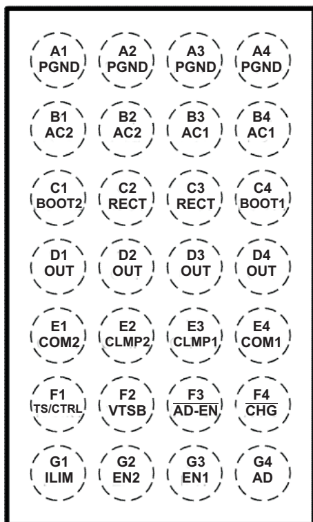
YFF Package (TOP VIEW)
