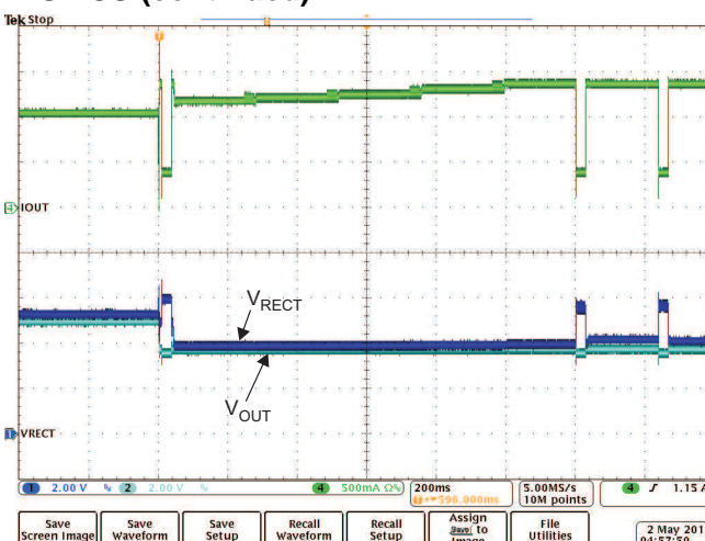
Figure 23. bq51011 Output Current Transition ( I_{LOAD} < I_{LIM} \geq I_{LOAD} = I_{LIM} ) Illustrating Dynamic Communication Current Limit
