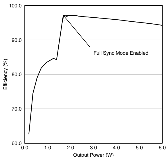
Figure 4. Rectifier Efficiency
