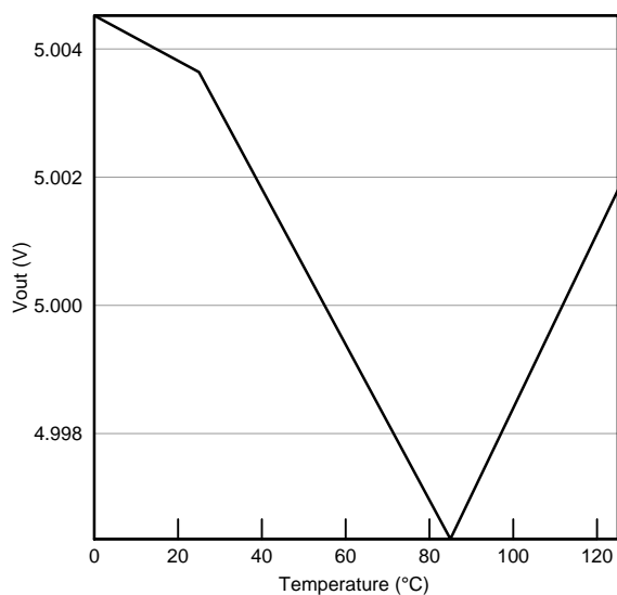
Figure 10. V_{OUT} vs Temperature
