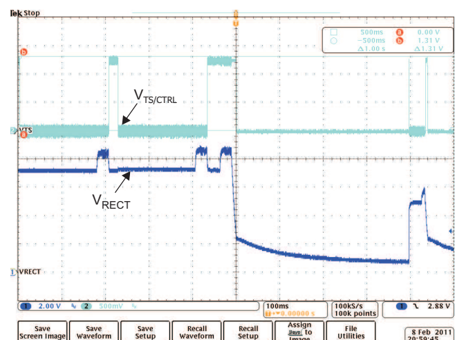
Figure 16. TS Fault
