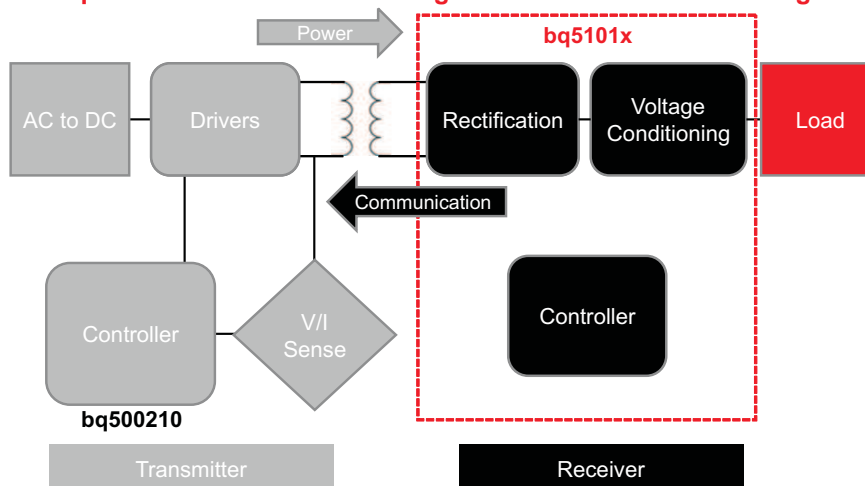
Figure 24. WPC Wireless Power System Indicating the Functional Integration of the bq5101x
