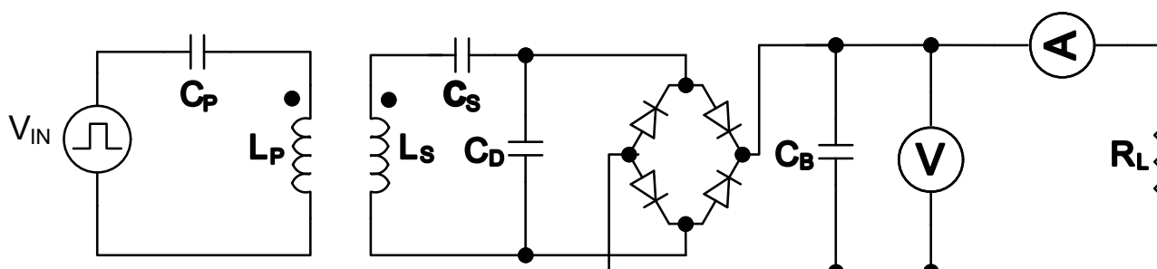
Figure 32. Load-Line Analysis Test Bench
