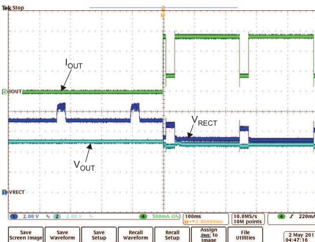
Figure 21. bq51011 Step Response with V_{OUT} = 4.8V and I_{LOAD} = I_{ILIM}
