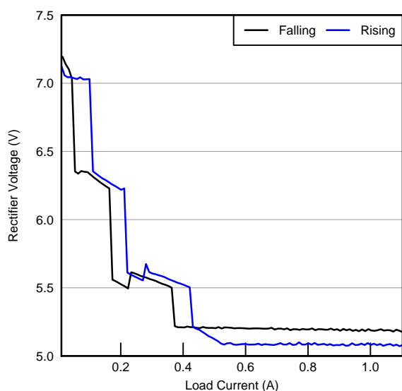
Figure 6. V_{RECT} vs. I_{LOAD}
