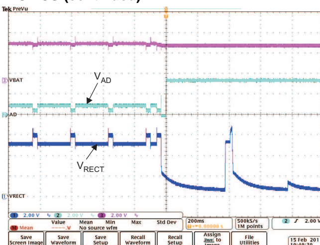
Figure 19. On the Go Enabled ( V_{OTG} = 3.5V )(3)
