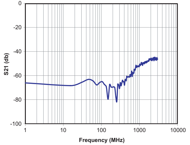
Analog Crosstalk
