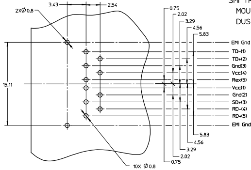
RECOMMENDED PCB LAYOUT DIMENSIONS TOLERANCE: ±0.1mm
