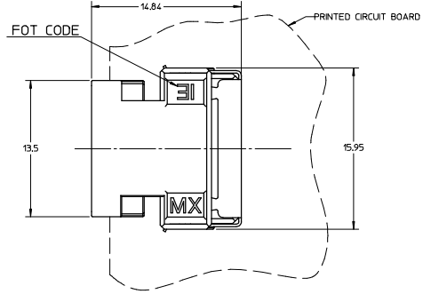
DUST CAP NOT SHOWN
