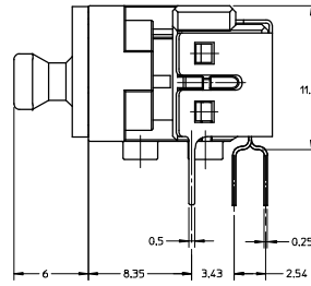
DUST CAP NOT SHOWN
