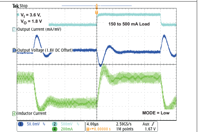
Figure 40. Load Transient Response in PWM/PWM Operation
