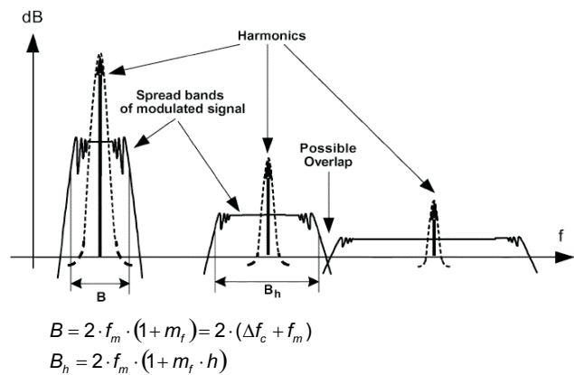
Figure 27. Spread Bands of Harmonics in Modulated Square Signals (1)
