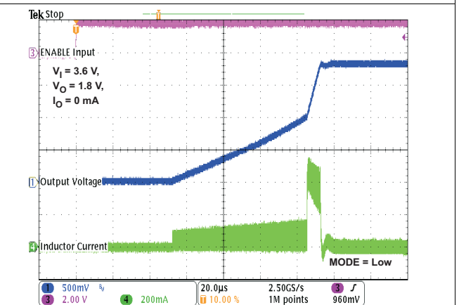
Figure 46. Start-Up
