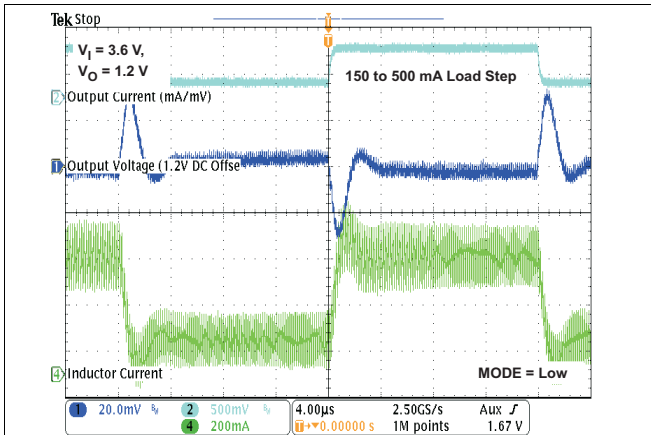
Figure 35. Load Transient Response in PWM/PWM Operation
