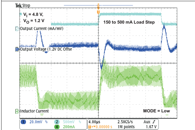
Figure 37. Load Transient Response in PWM/PWM Operation
