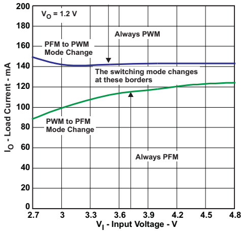
Figure 13. PFM/PWM Boundaries
