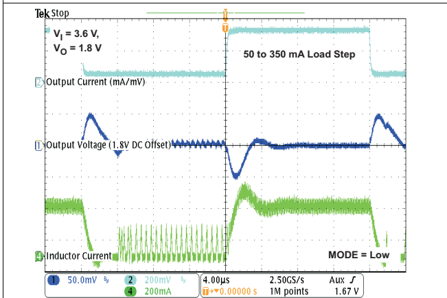
Figure 39. Load Transient Response in PFM/PWM Operation
