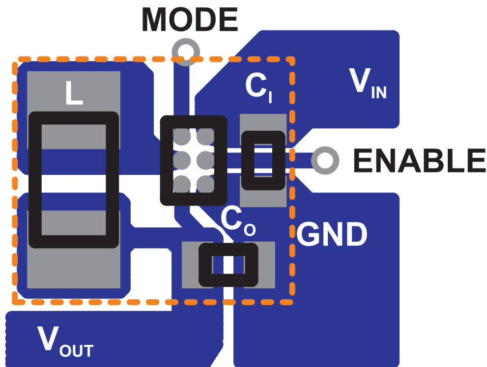
Figure 53. Suggested Layout (Top)
