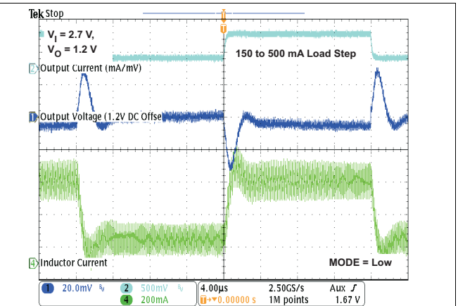
Figure 36. Load Transient Response in PWM/PWM Operation
