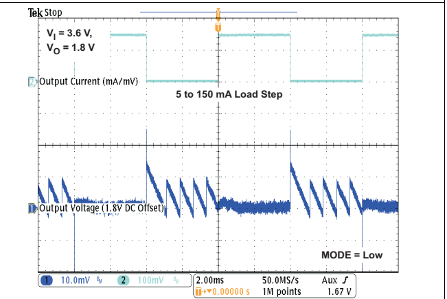
Figure 38. Load Transient Response in PFM/PWM Operation
