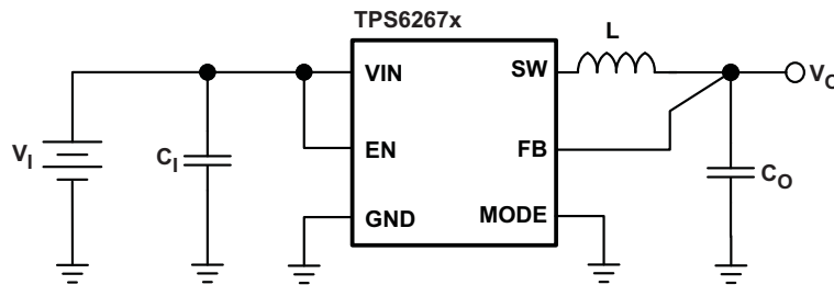
Figure 24. Measurement Setup
