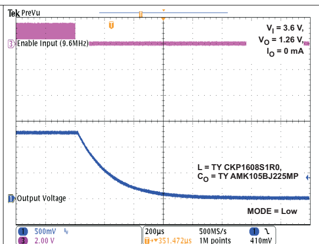
Figure 52. Shut-Down (RF Clock)
