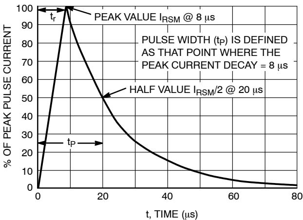
Figure 1. 8 \times 20 \mu s Pulse Waveform
