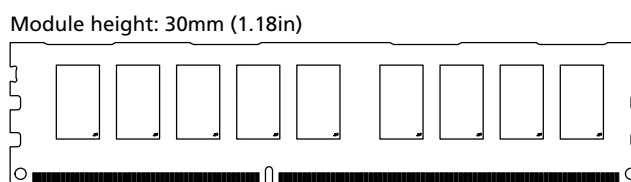
Figure 1: 240-Pin UDIMM (MO-269 R/C E)
