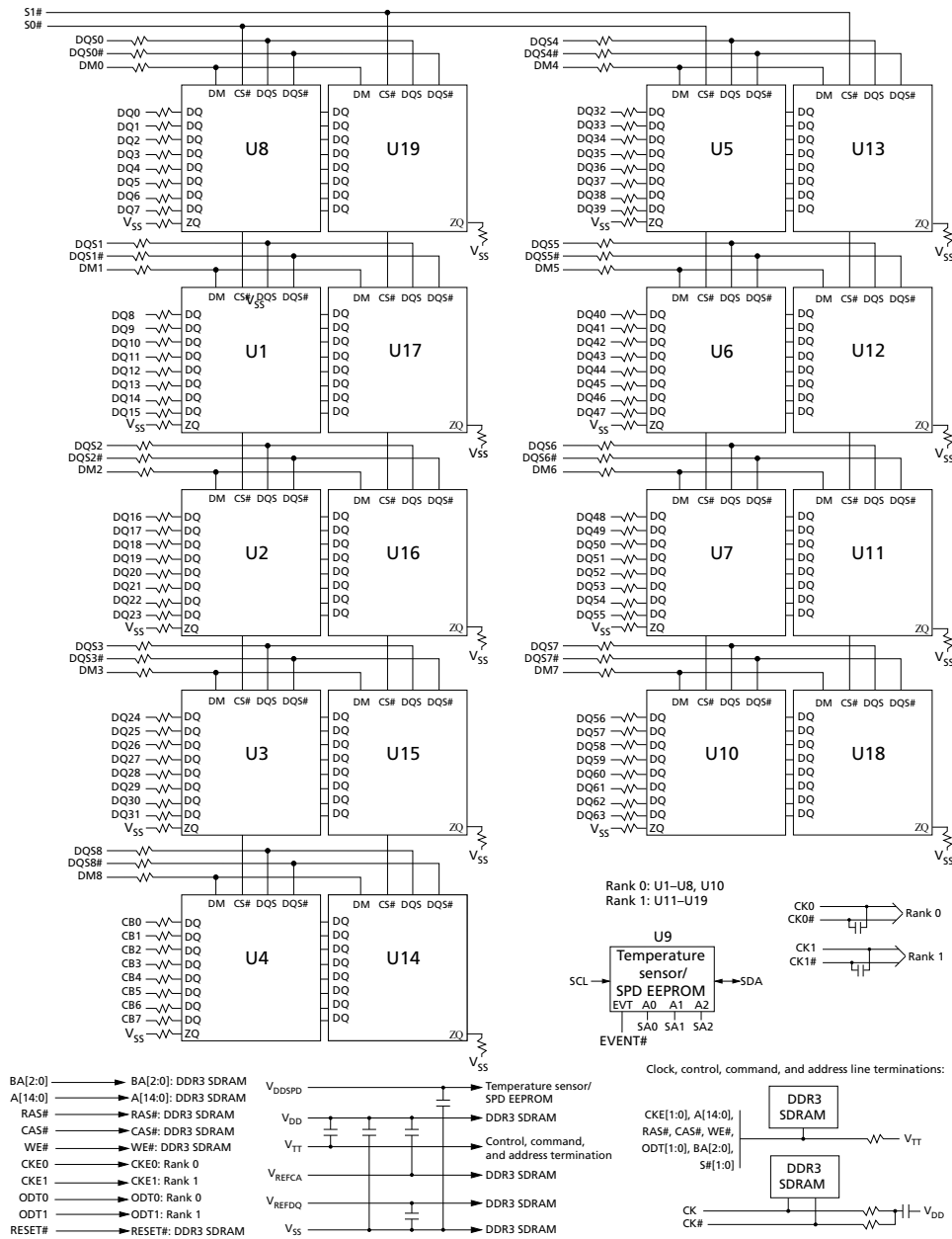
Figure 2: Functional Block Diagram
